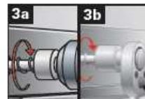
3a 3b Tighten the concrete screw with a socket spanner (spanner size 15). Observe the maximum tightening torques.
