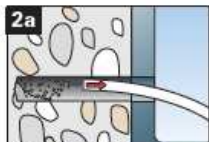
2a Clean drill hole
